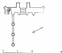
PLAN AA
